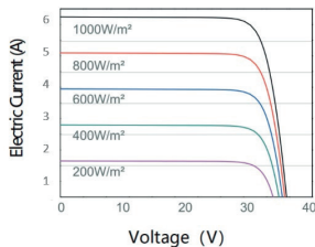
Current Voltage Curve
