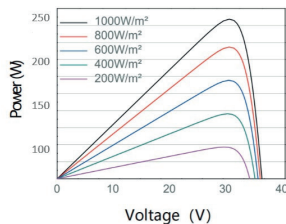
Power Voltage Curve
